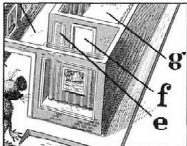
Confused labels
